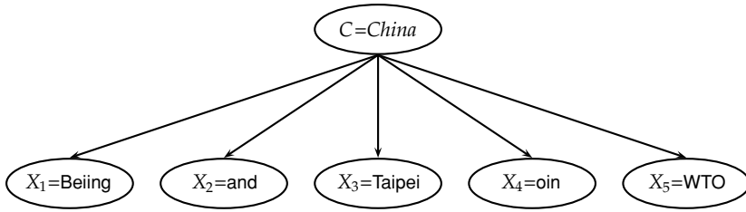
Figure 13.4 The multinomial NB model.
