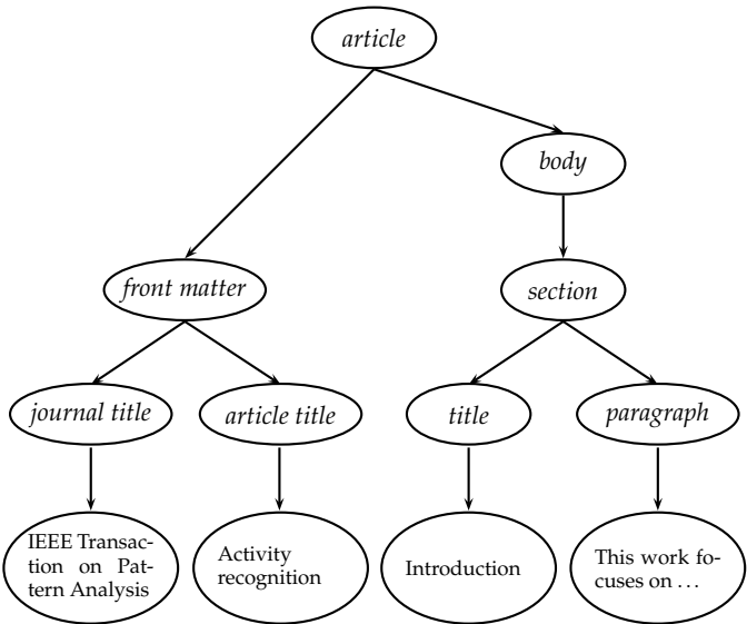
Figure 10.11 Simplified schema of the documents in the INEX collection.
