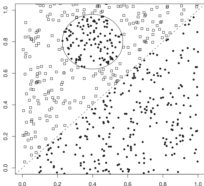
Figure 14.11 A nonlinear problem.
