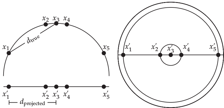
Figure 14.2 Projections of small areas of the unit sphere preserve distances. Left: A projection of the 2D semicircle to 1D. For the points x_1, x_2, x_3, x_4, x_5 at x coordinates -0.9, -0.2, 0, 0.2, 0.9 the distance |x_2x_3| \approx 0.201 only differs by 0.5% from |x'_2x'_3| = 0.2 ; but |x_1x_3|/|x'_1x'_3| = d_{\text{true}}/d_{\text{projected}} \approx 1.06/0.9 \approx 1.18 is an example of a large distortion (18%) when projecting a large area. Right: The corresponding projection of the 3D hemisphere to 2D.
