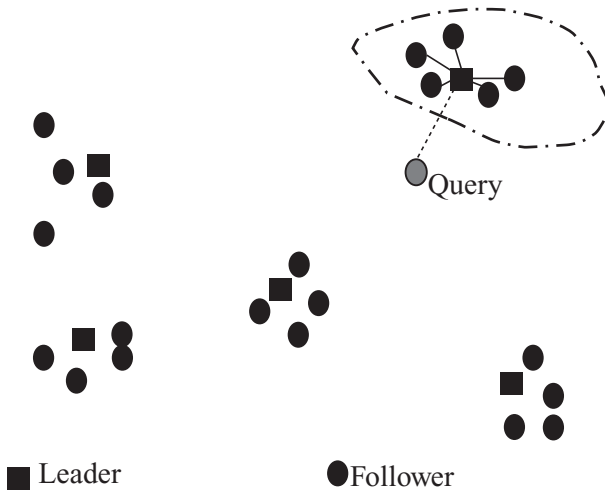
Figure 7.3 Cluster pruning.
