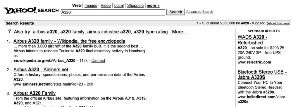
Figure 19.6 Search advertising triggered by query keywords. Here the query A320 returns algorithmic search results about the Airbus aircraft, together with advertisements for various non-aircraft goods numbered A320 that advertisers seek to market to those querying on this query. The lack of advertisements for the aircraft reflects the fact that few marketers attempt to sell A320 aircraft on the web.
