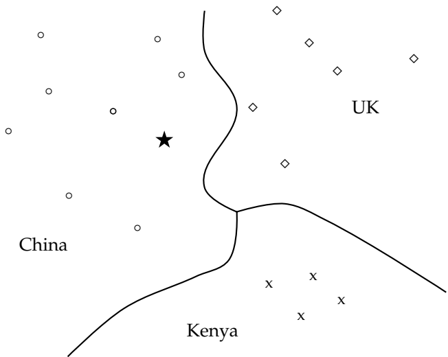
Figure 14.1 Vector space classification into three classes.
