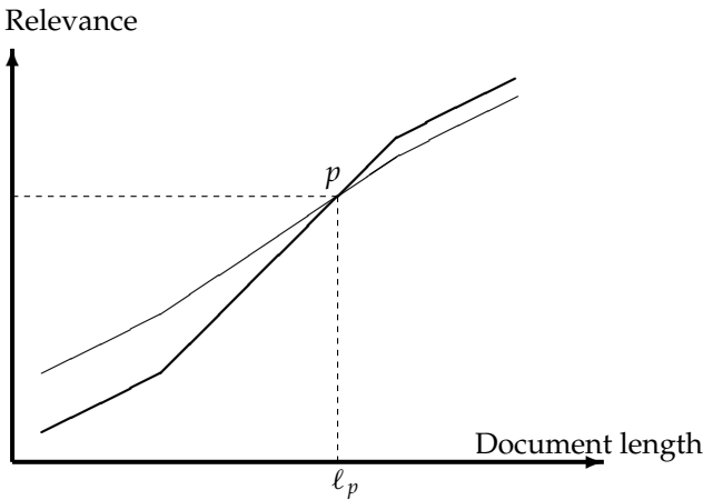
Figure 6.16 Pivoted document length normalization.
