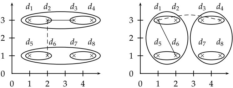
Figure 17.4 A single-link (left) and complete-link (right) clustering of eight documents. The ellipses correspond to successive clustering stages. Left: The single-link similarity of the two upper two-point clusters is the similarity of d_2 and d_3 (solid line), which is greater than the single-link similarity of the two left two-point clusters (dashed line). Right: The complete-link similarity of the two upper two-point clusters is the similarity of d_1 and d_4 (dashed line), which is smaller than the complete-link similarity of the two left two-point clusters (solid line).
