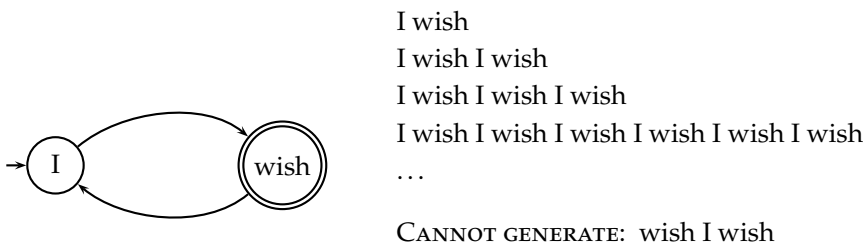
Figure 12.1 A simple finite automaton and some of the strings in the language it generates. \rightarrow shows the start state of the automaton and a double circle indicates a (possible) finishing state.
